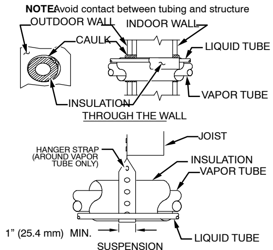
Fig. 1 - Piping Installation
