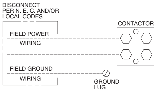
Fig. 6 - Line Connections
