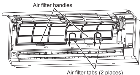
Air filter tabs (2 places)
